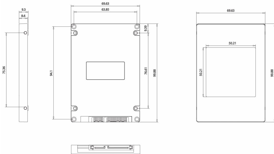
Figure 5: FiD 2.5 SATA4000 mechanical dimensions
