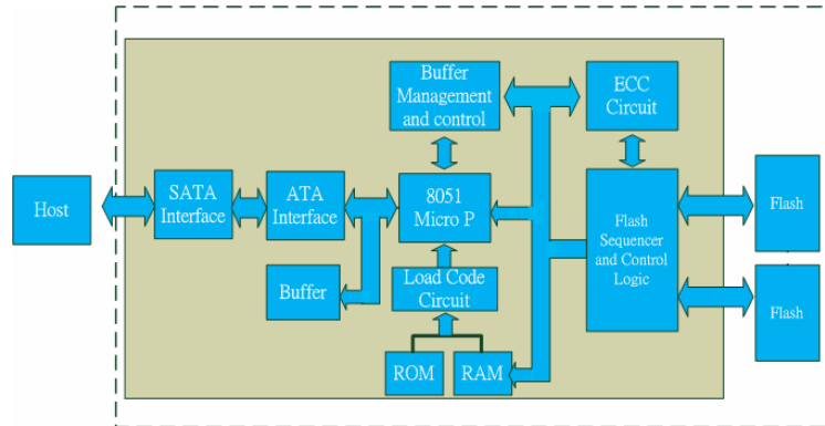
Figure 2: InnoDisk FiD 2.5" SATA4000 Block Diagram
